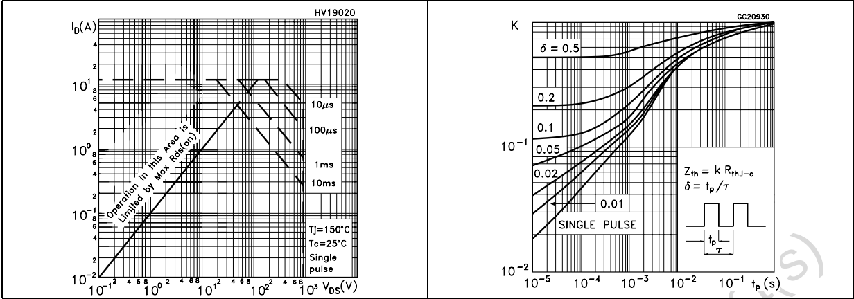
Figure 3. Safe operating area for TO-220FP
